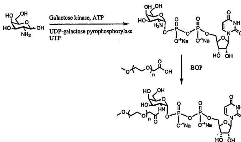
Scheme 11
